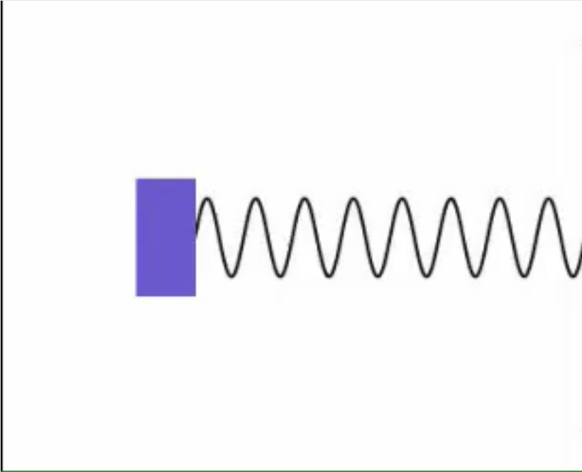
[ harmonic oscillation ]
