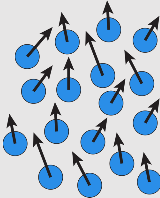
[ Lagrangian ]
